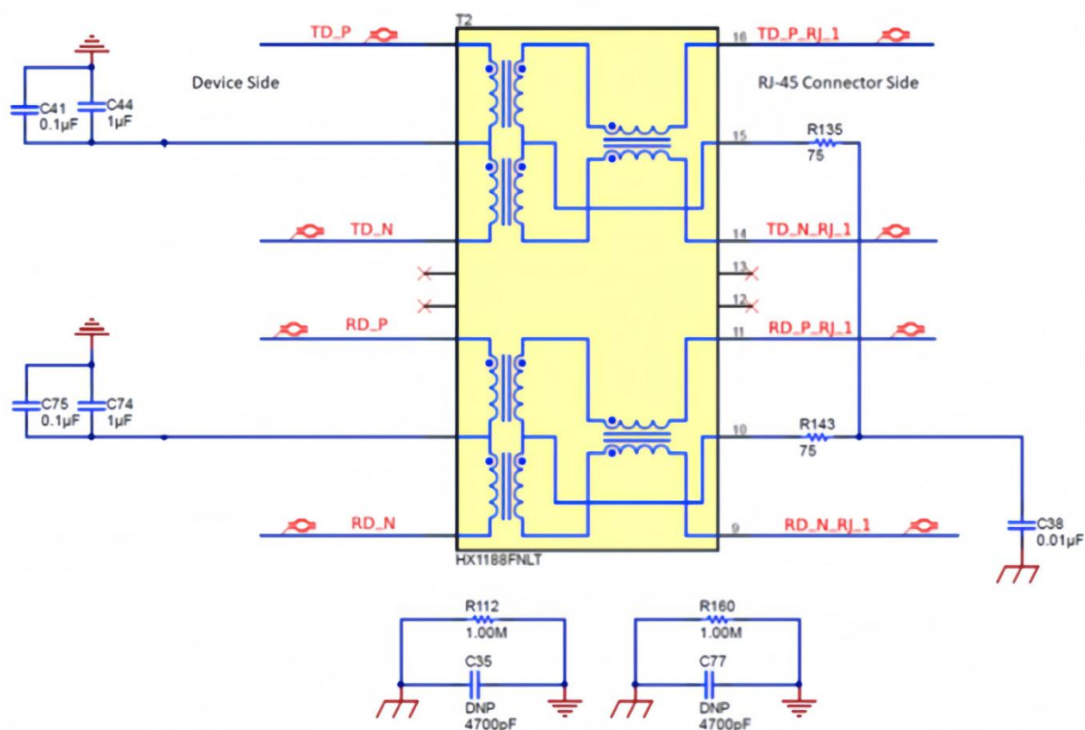
Figure 6. Transformer Connection Mode of K922 / K922 接变压器方式
